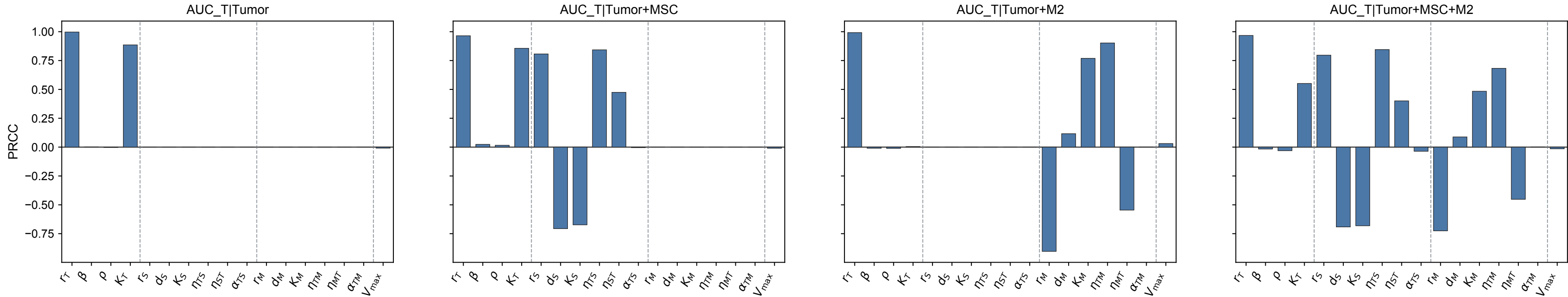
OVCA3: PRCC on AUC of Tumor cells T(t)
